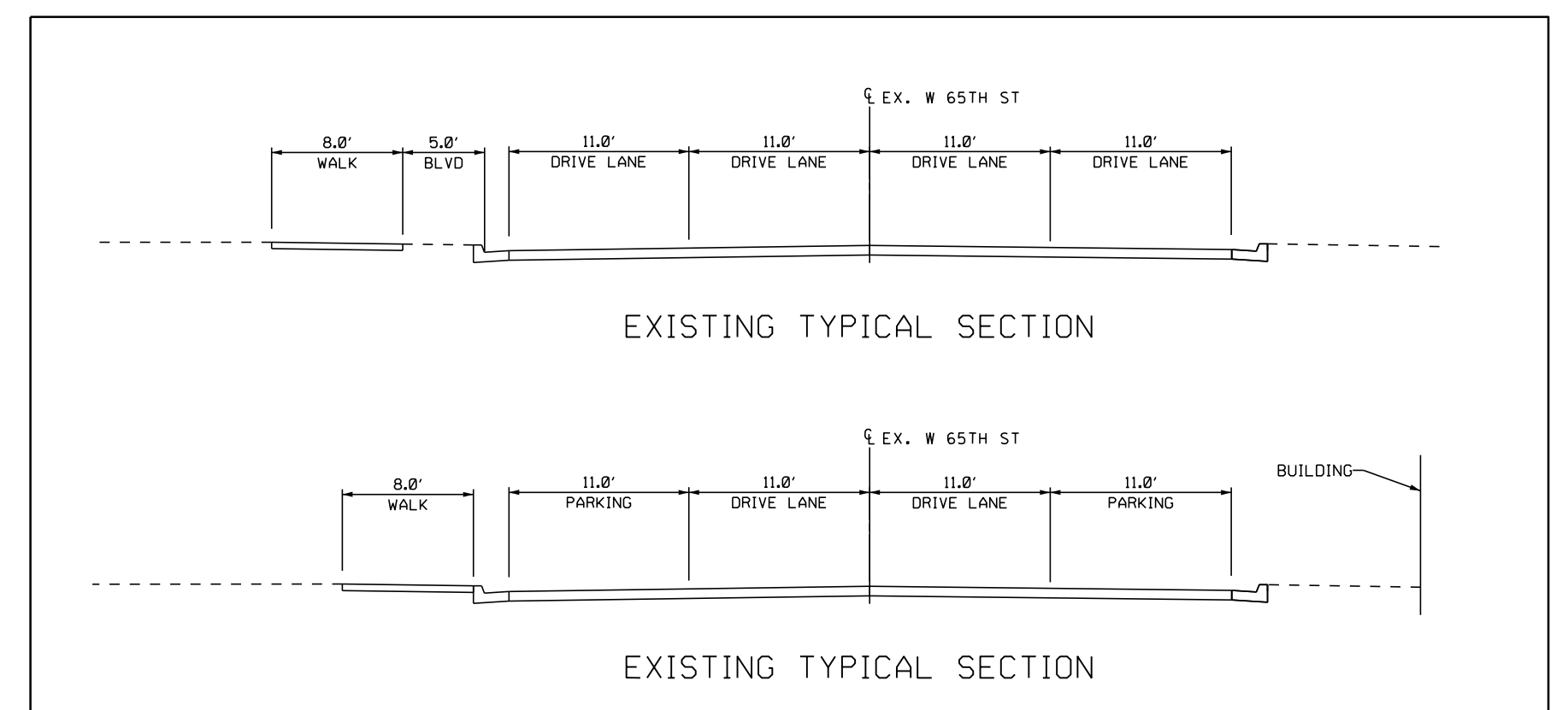
EXISTING TYPICAL SECTION
