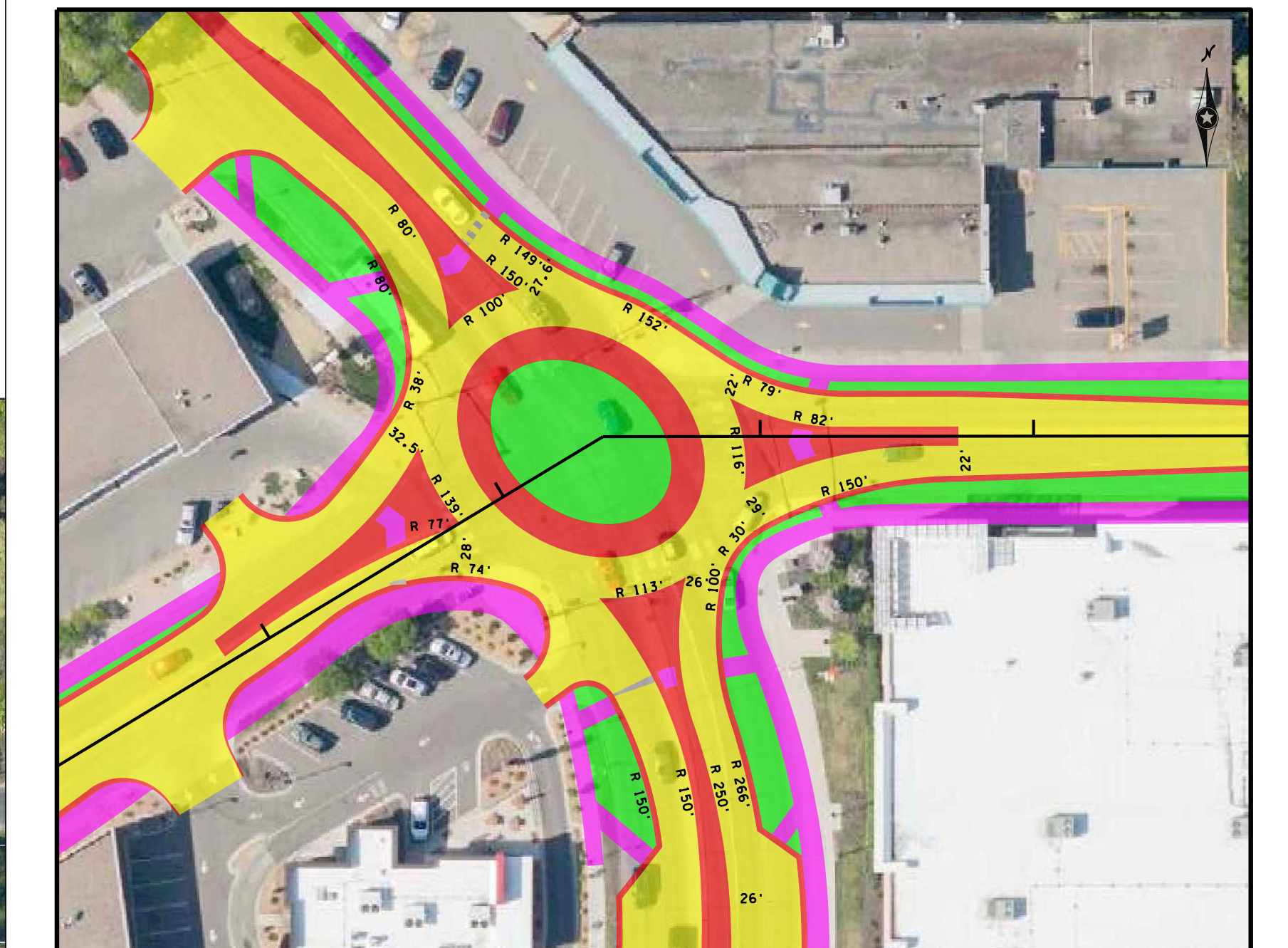
W 66TH ST & LYNDALE AVE ROUNDAABOUT
