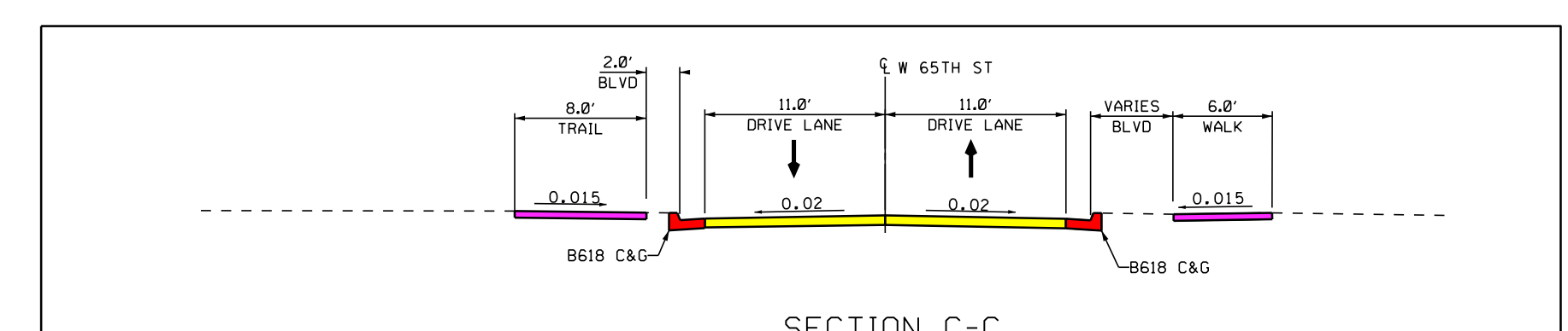
SECTION C-C
