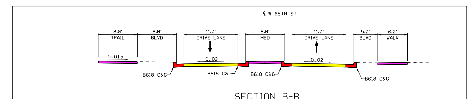
SECTION B-B
