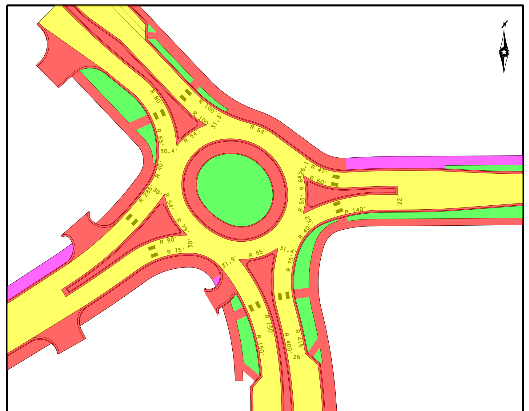
INSET A W 65TH ST & LYNDALE AVE ROUNDABOUT ROTONDA DE W 65TH STREET & LYNDALE AVENUE
